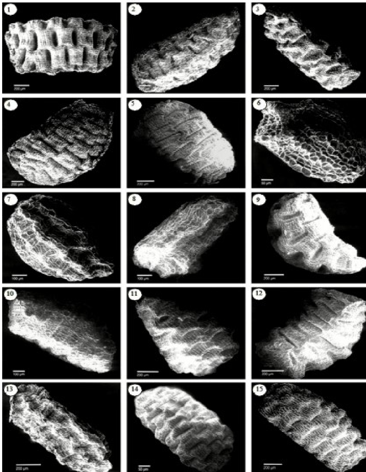
Figures 1-15. Alveolate types. 1. S. pruinosa 1 (far deeply). 2. S. azerbaijanica (deeply). 3. S. deserti (shallowly). 4, 5. ridged type: 4. S. leucoclada (far deeply) and as the largest seed, 5. S. striata 2 (deeply). 6-8. without alveoli or ridges type and sometimes longitudinally undulate: 6. S. chlorantha (as the smallest seed). 7, 8. S. umbrosa 1, 2 . 9. S. pruinosa 3 , 10. S. frigida subsp. haussknechtii 2 . 11. S. frigida subsp. frigida 2 . 12. S. frigida subsp. frigida 1 . 13. S. variegata subsp. cinerascens . 14. S. variegata subsp. variegata . 15. S. variegata subsp. rupestris
