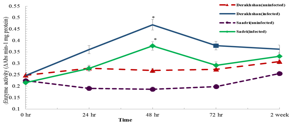
Fig 4. Changes in Proxidase enzyme activity of (ΔAbs min -1 mg protein) in Sadri and Derakhshan varieties at 0, 24, 48, 72, and 2 weeks after inoculation of the pathogen bacteria. Each point represents the mean of four replications ± standard error (SE). ** Significant at P < 0.01, * Significant at P < 0.05.
